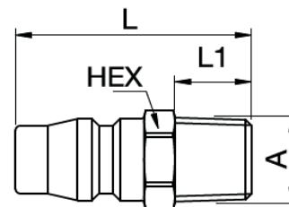
Male Thread
